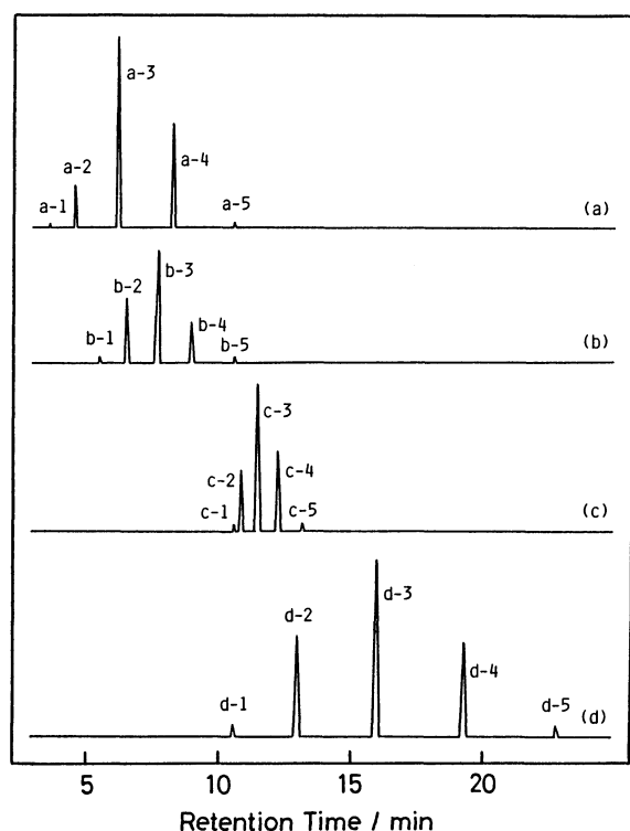
Fig. 1. Gas chromatograms of the products obtained by treating the TAOS-HMDS solutions at the HMDS/TAOS ratio of 4.0 with Amberlyst 15 at 40^\circ\text{C} for 85 h. TAOS: (a) TMOS, (b) TEOS, (c) TPOS, and (d) TBOS.
